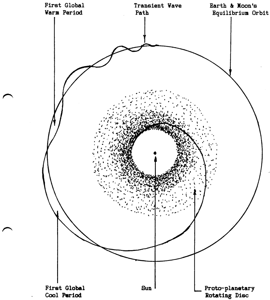
Earth and Moon Evolutionary Path in Reverse Model of Planetary Evolution
